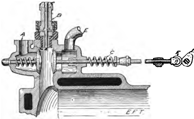
FIG. 283.—Detail Diagram of the Valves and Attachments of a Gas Engine Cylinder. A is the inlet port behind inlet valve held in its seat by a tension spring; B, the spark plug for "jump-spark" ignition; C, the push rod and compression spring of the exhaust valve; D, the cam opening the exhaust; E, the exhaust port; F, the roller at end of valve rod bearing on the cam, D.
